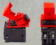
5340-00-NIB-0393 Clamp-On Breaker Lockout with Cleat, 480/600V
